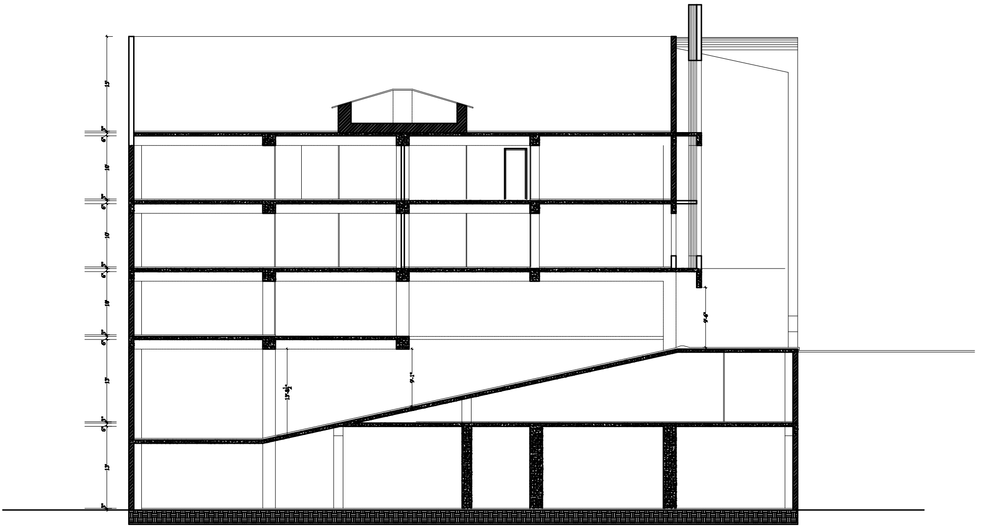
X-SECTION OF A-A
